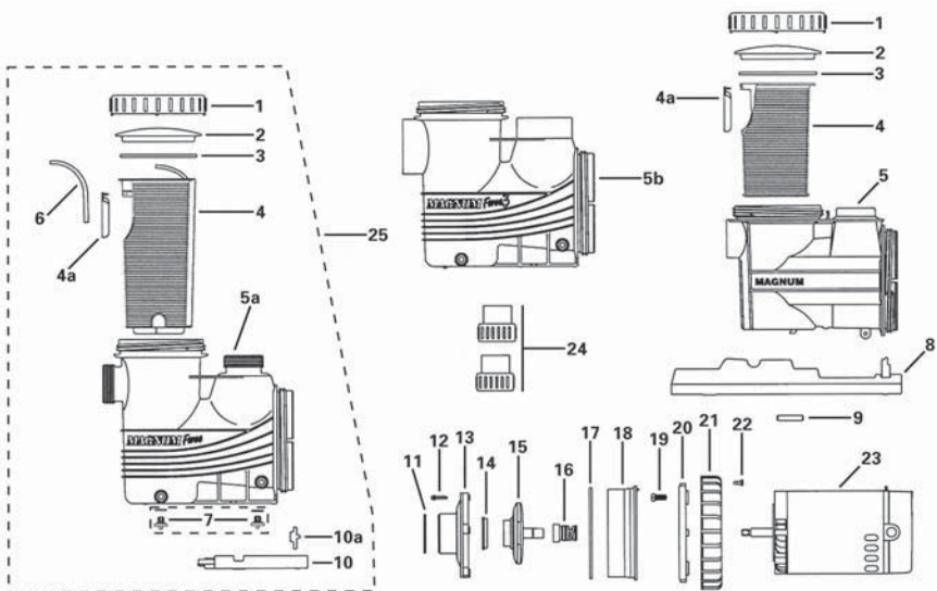
Parts for Models Magnum, Magnum Plus, Magnum Force & Magnum Force 3
